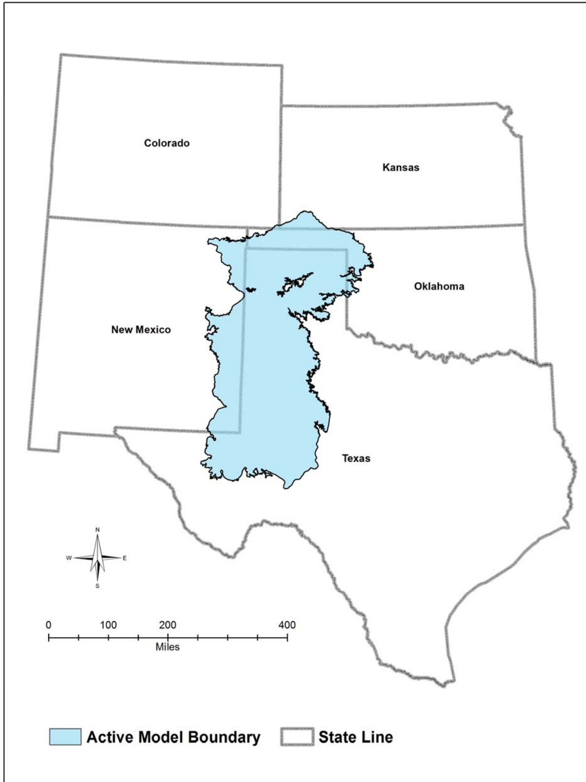
Figure 2.0.1 Study area for the High Plains Aquifer System groundwater availability model.
