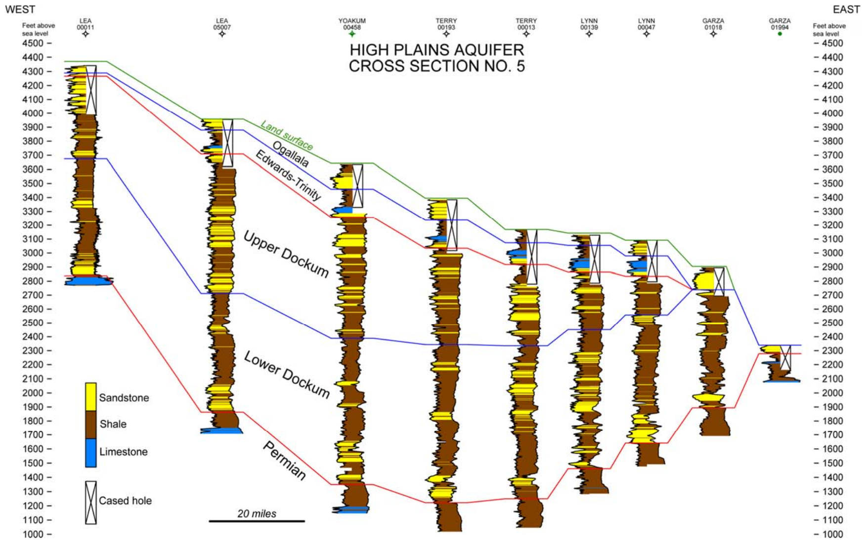
Figure 4.2.7 Cross-section #5.
