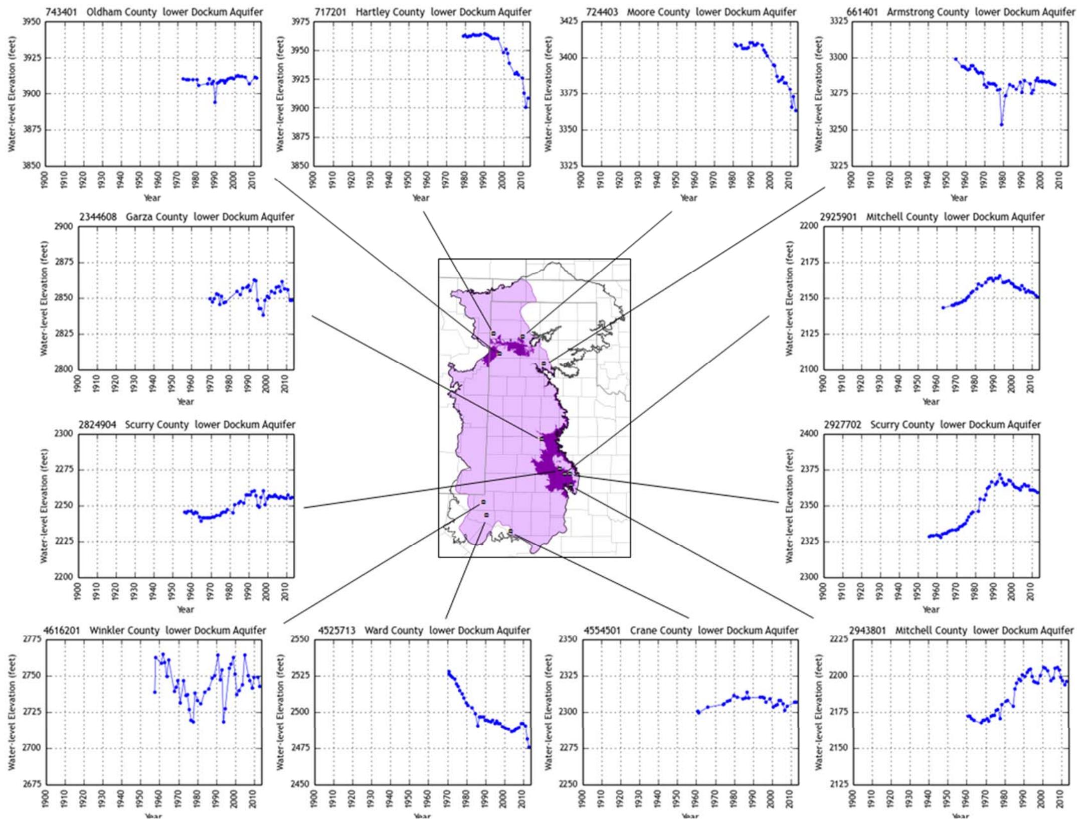
Figure 4.3.24 Select hydrographs for wells completed into the lower Dockum Aquifer.
