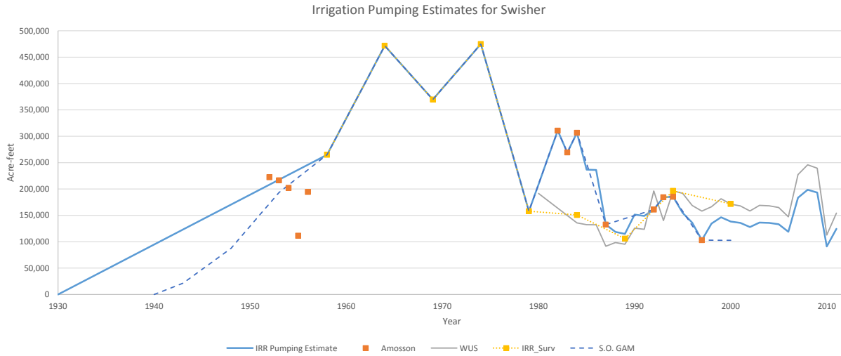
Figure 4.7.16 Comparison of estimated irrigation pumping for Swisher County between the current model, the Amosson and others (2003) data, the TWDB water use survey data , the TWDB irrigation survey data (TWDB, 1991), and the pre-calibrated/no return flow pumping estimates from the original Southern Ogallala Aquifer groundwater availability model (Blandford and others, 2003).
